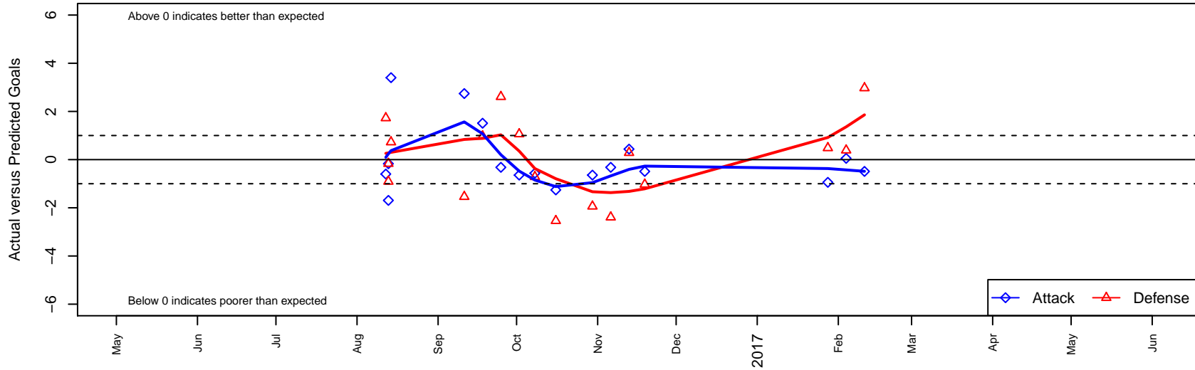
TC United Navy B98 Dots are actual minus expected GF (blue circles) and GA (red triangles). Blue line is smoothed change in attack strength. Red is smoothed change in defense strength.
